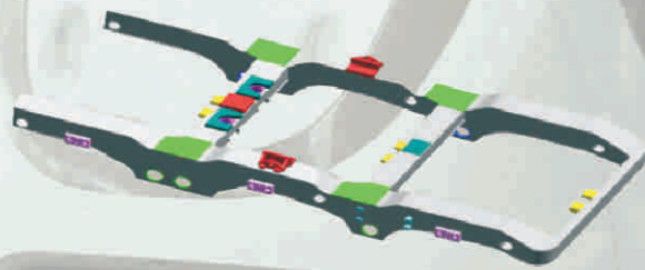
Fabricated Bogie Frame
