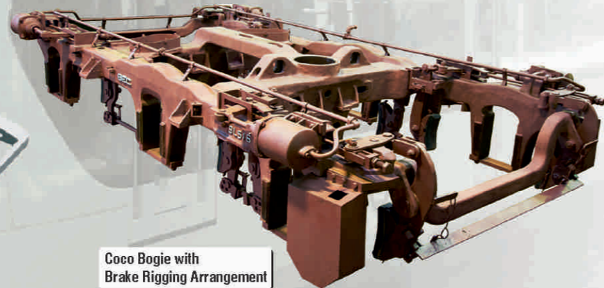
Locomotive Flexi-Coil Bogie
