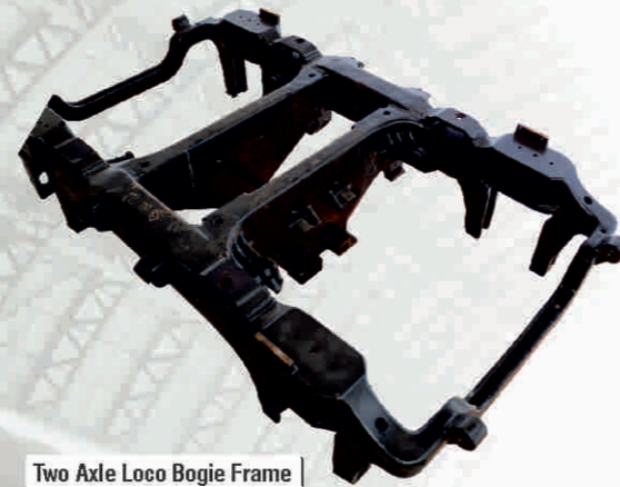
Two Axle Loco Bogie Frame
