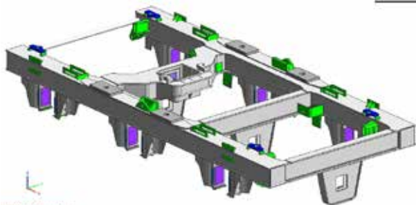
Bogie frame for WDM 3D Locomotives
