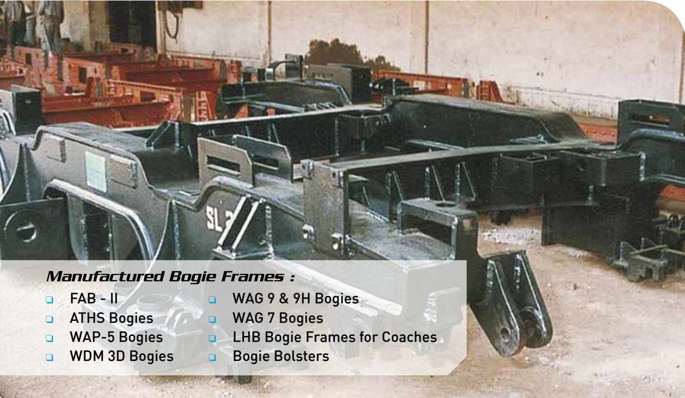
Bogie frame (FAB - II) for WDP 4 & WDG 4 Locomotives
