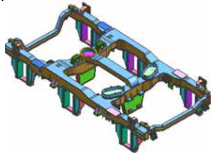
Fabricated Bogie frame for Conventional and Advanced Railway Coaches
