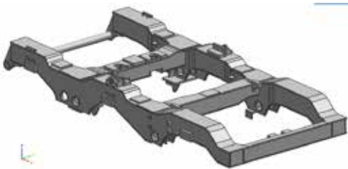
Bogie frame (FAB - II) for WDP 4 & WDG 4 Locomotives
